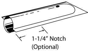
Welded Type I.D. = Nominal Dia. + 1/8"
